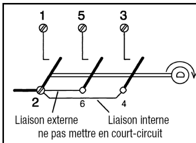
Raccordement
