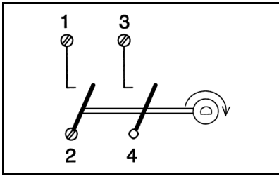
Raccordement
