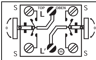
Contact assignments
