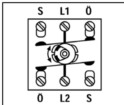
Contact assignments
