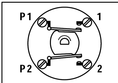
Contact assignments
