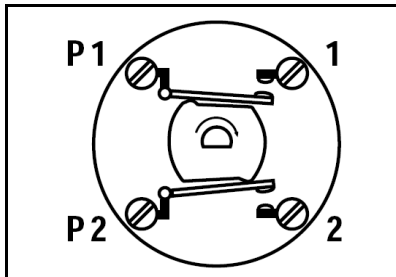
Contact assignments
