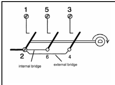
Contact assignments
