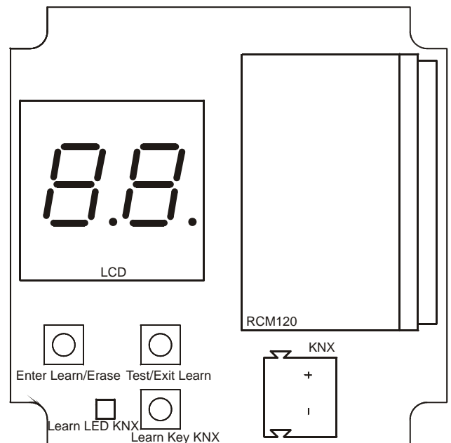
Figure 2: Device with top open
