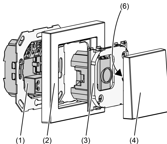
Figure 2: Device fitting
