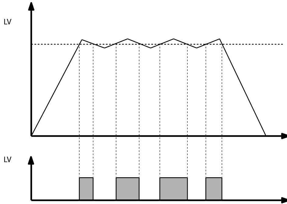
Figure 13: Frequency of switching without hysteresis
