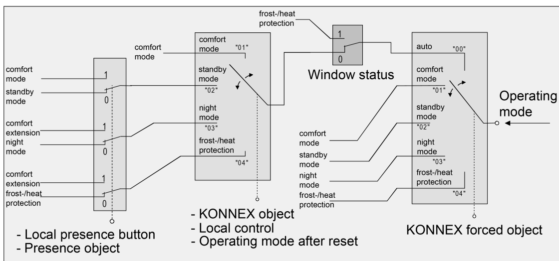
Figure 28: Operating mode change-over through KONNEX object with presence button
