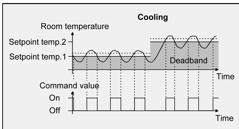
Figure 23: 2-point feedback control for mixed "Heating and cooling" mode with active cooling operation.
