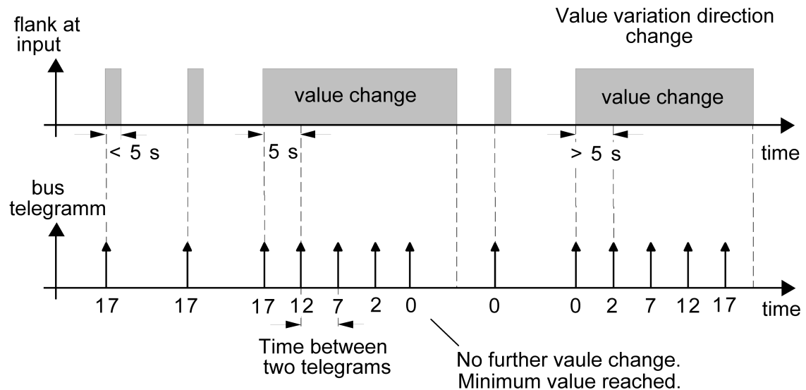
Figure 10: Example to change the value for dimming value transmitter
