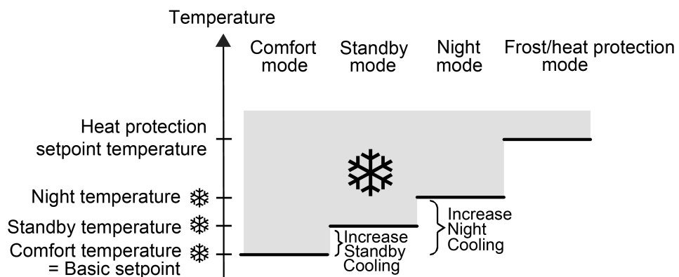
Figure 32: Setpoint temperatures in the operating mode "Cooling"
