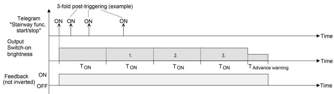
Figure 47: Time extension of the staircase function
